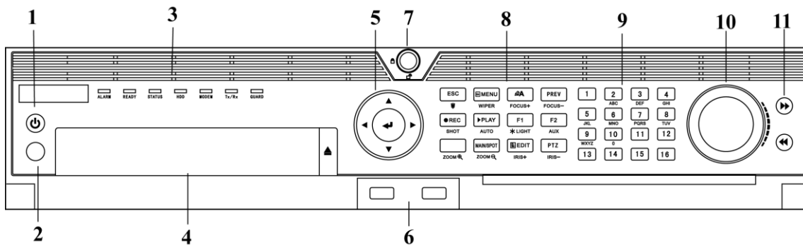
Figure 1-5 Front Panel
