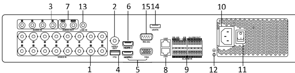
Figure 1-11 Rear Panel
