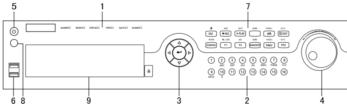
Figure 1-4 Front Panel
