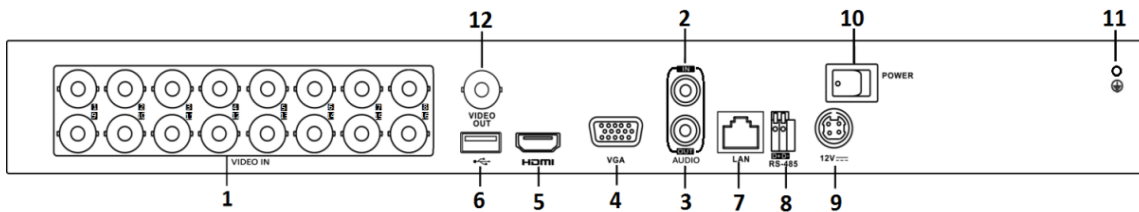
Figure 1-9 Rear Panel
