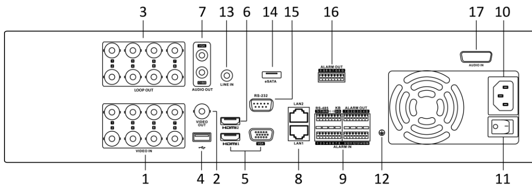
Figure 1-12 Rear Panel
