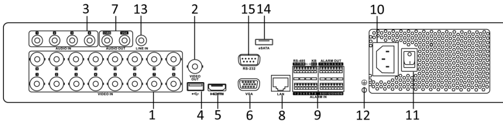
Figure 1-10 Rear Panel
