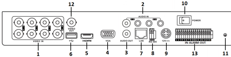
Figure 1-8 Rear Panel
